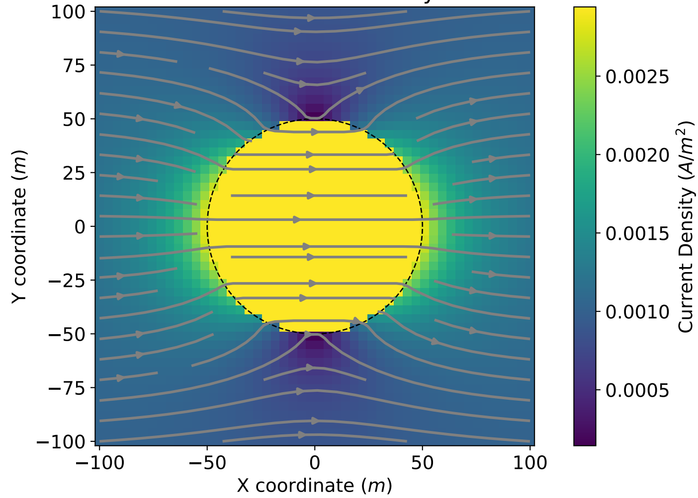
Conductive Sphere: Secondary Current Density
