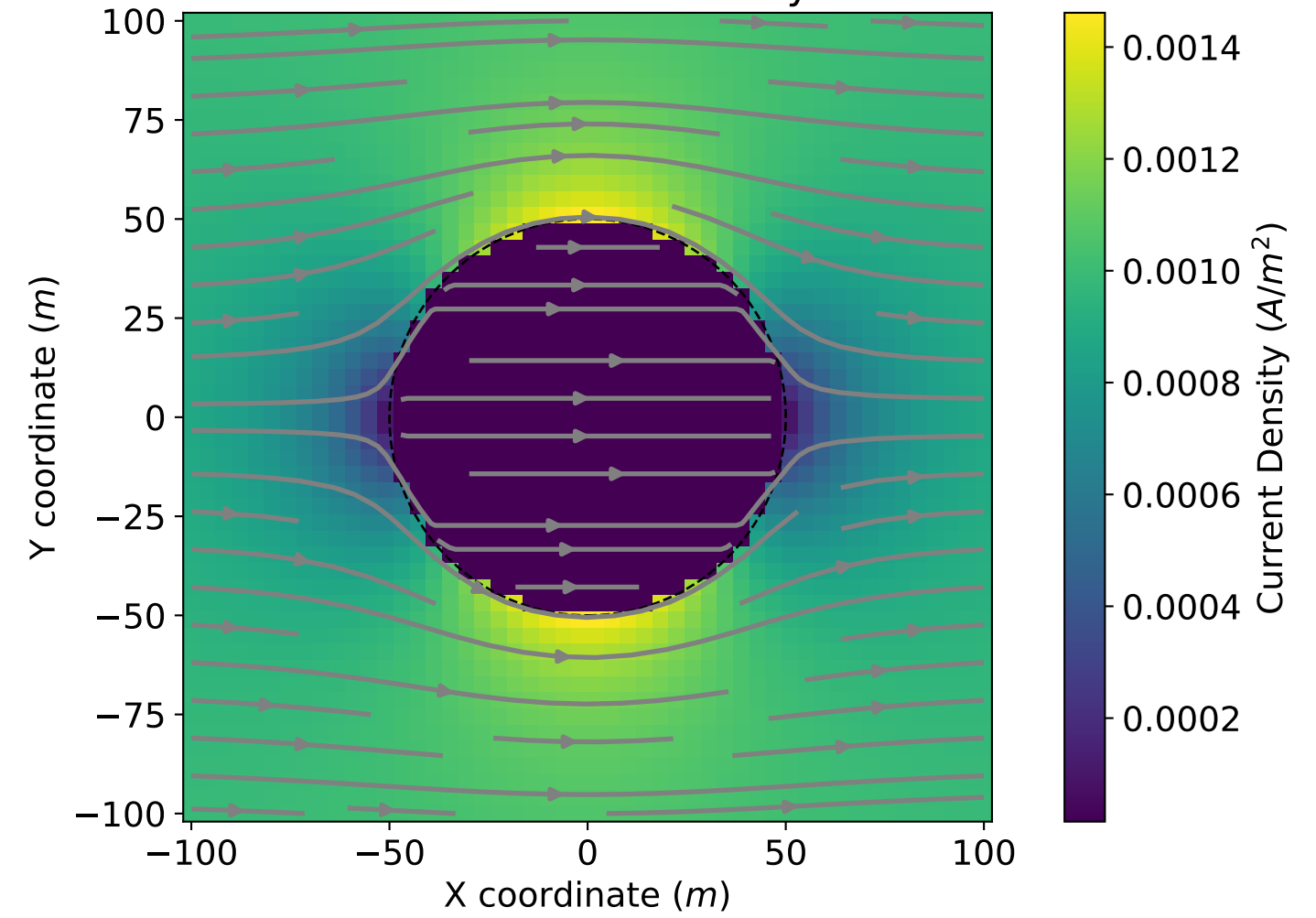
Resistive Sphere: Secondary Current Density
