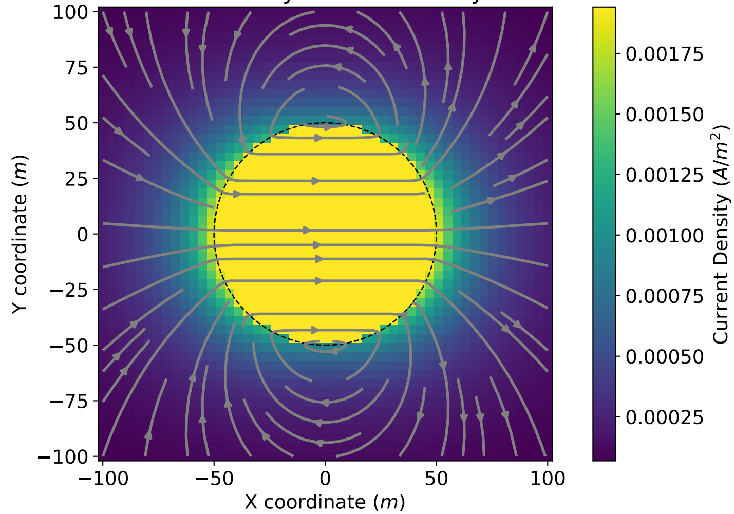
Conductive Sphere: Secondary Current Density
