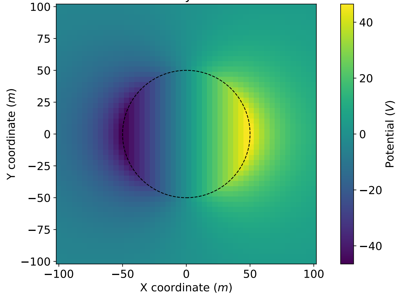
Conductive Sphere: Secondary Potential
