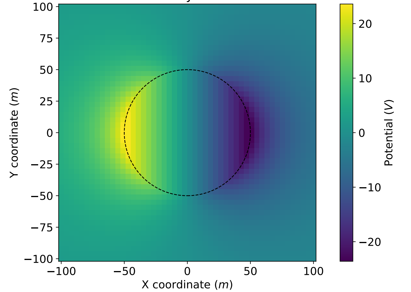
Resistive Sphere: Secondary Potential
