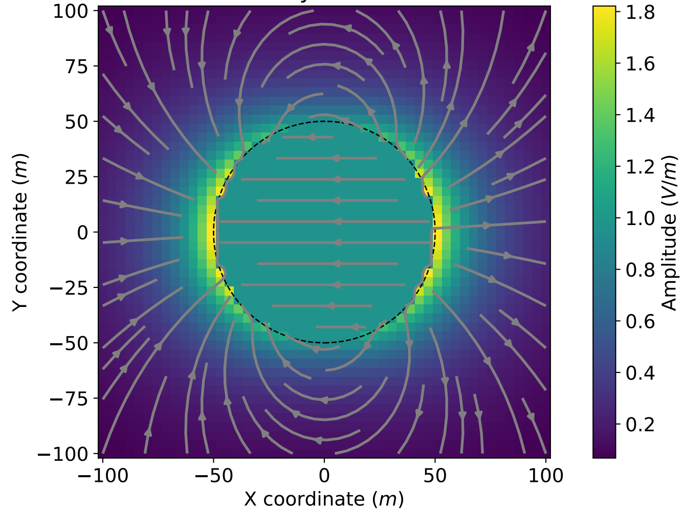
Conductive Sphere: Secondary Electric Field
