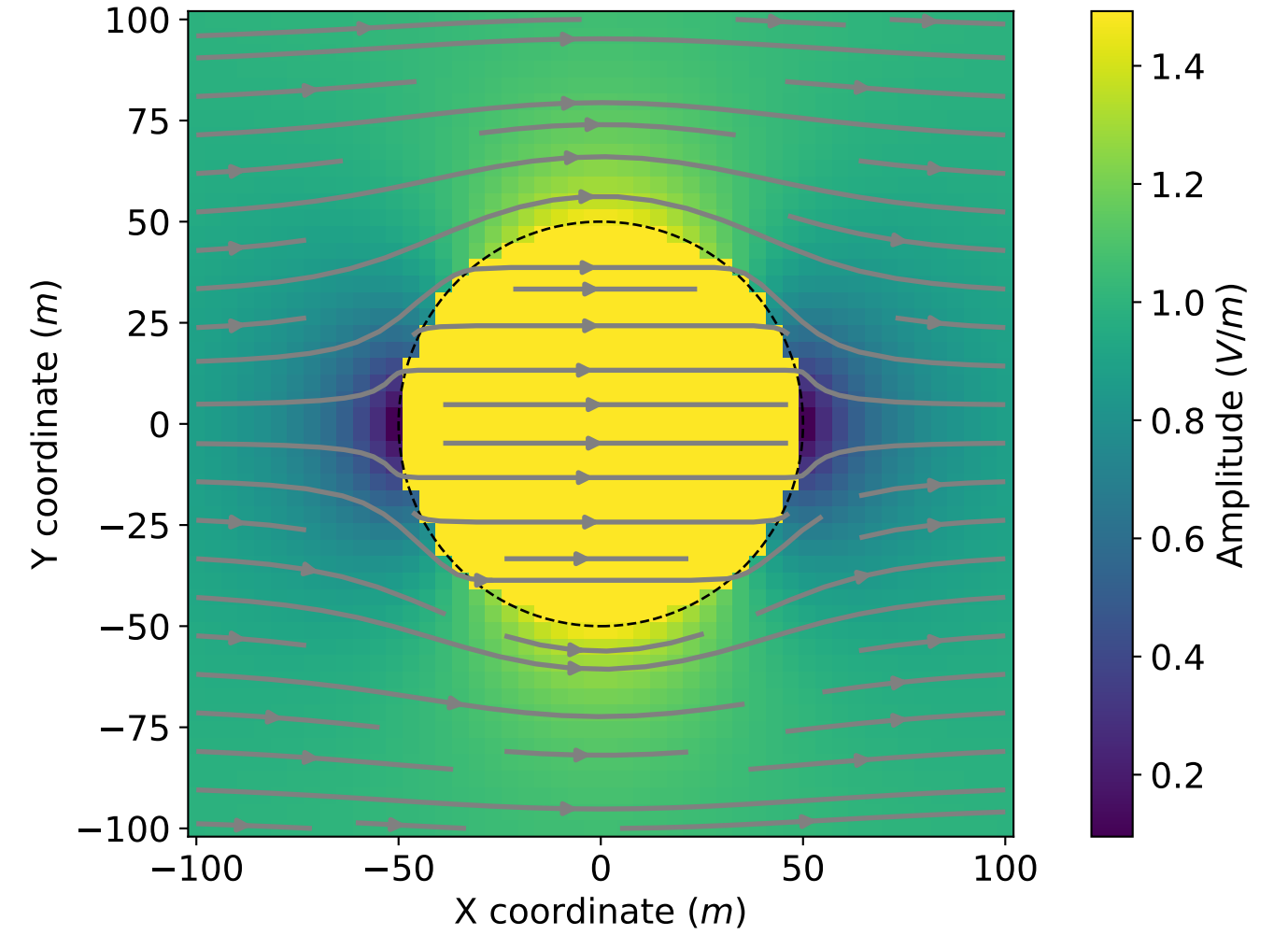
Resistive Sphere: Secondary Electric Field
